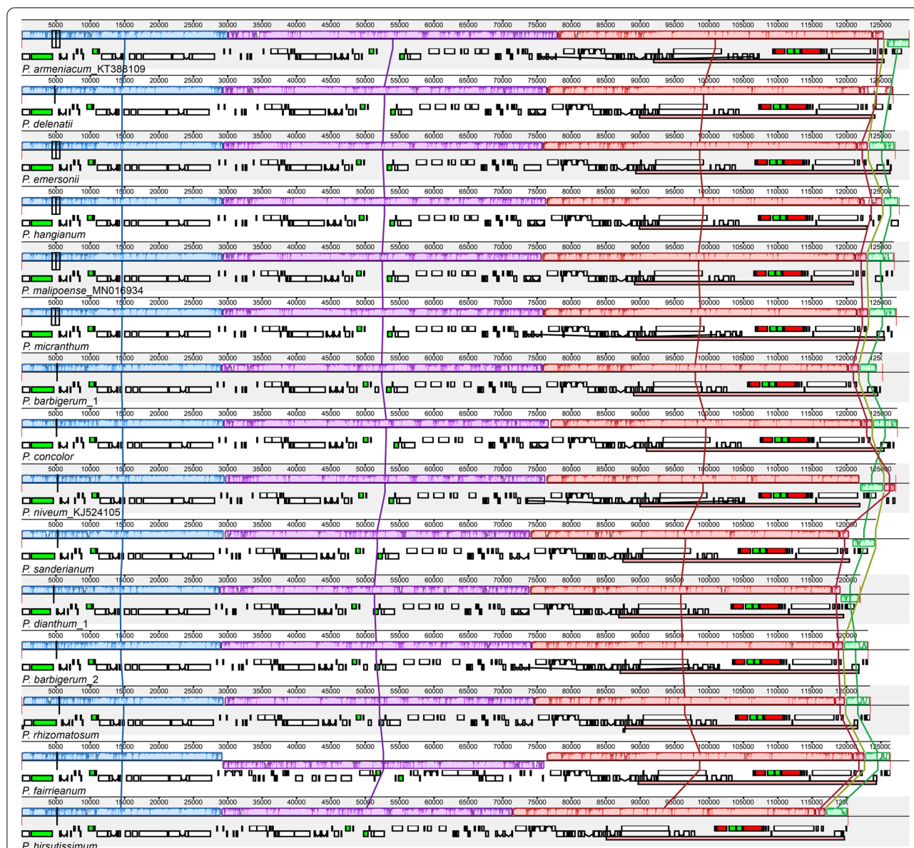
Fig. 3 Extent of the gene rearrangements of 15 Paphiopedilum chloroplast genomes. Locally collinear blocks of the sequences are colour-coded and connected by lines
