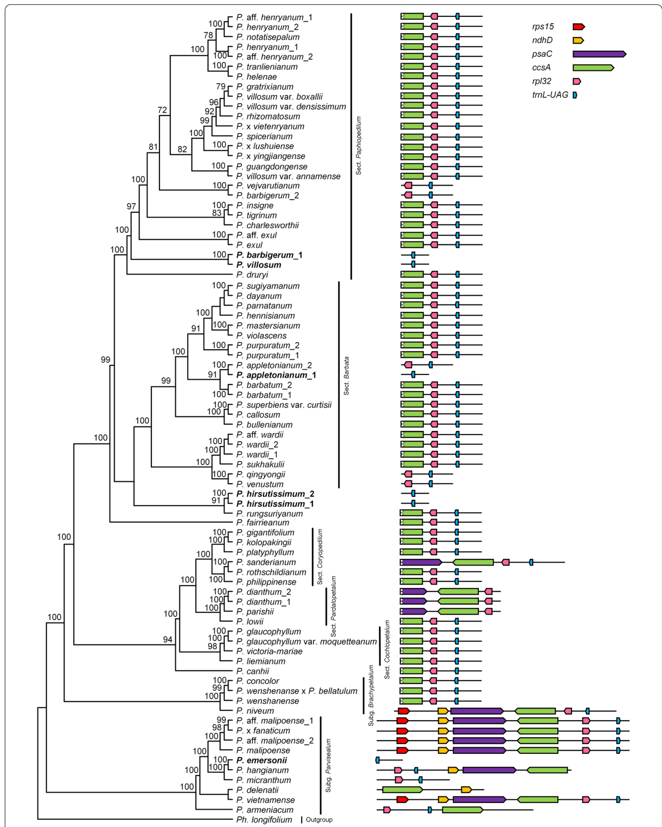
Fig. 2 The variation in SSC regions of Paphiopedilum . The scaled representations of SSC types are plotted on the ML tree. The five species in bold lost all the functional ndh genes
