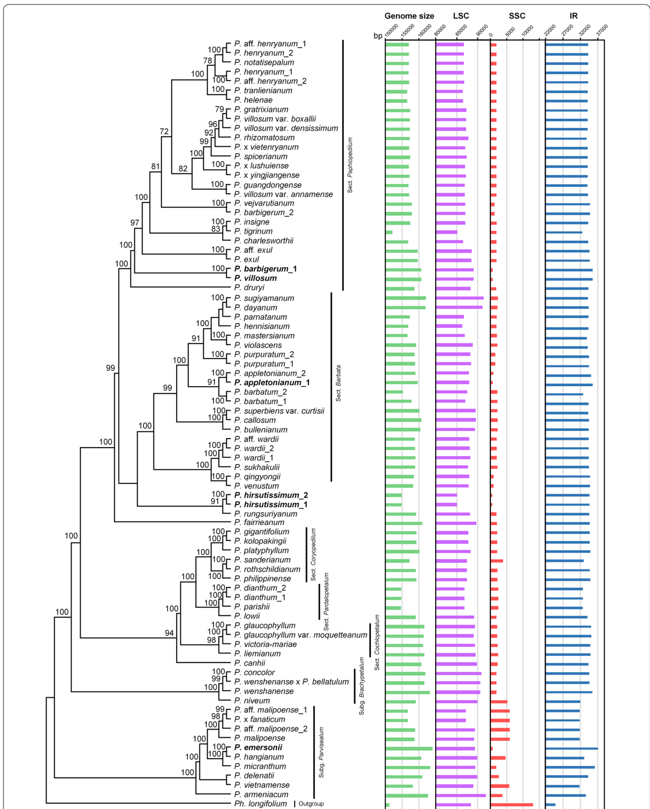
Fig. 1 The length of plastid genome size, LSC, SSC, and IR regions were plotted on the ML tree of Paphiopedilum . LSC, SSC, and IR regions were scaled differently. The six samples in bold only have trnL-UAG preserved in the SSC region
